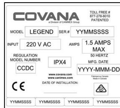
Specification label, located on the AC control box Note: This label provides the serial number (For AC operated model only, European Only)
